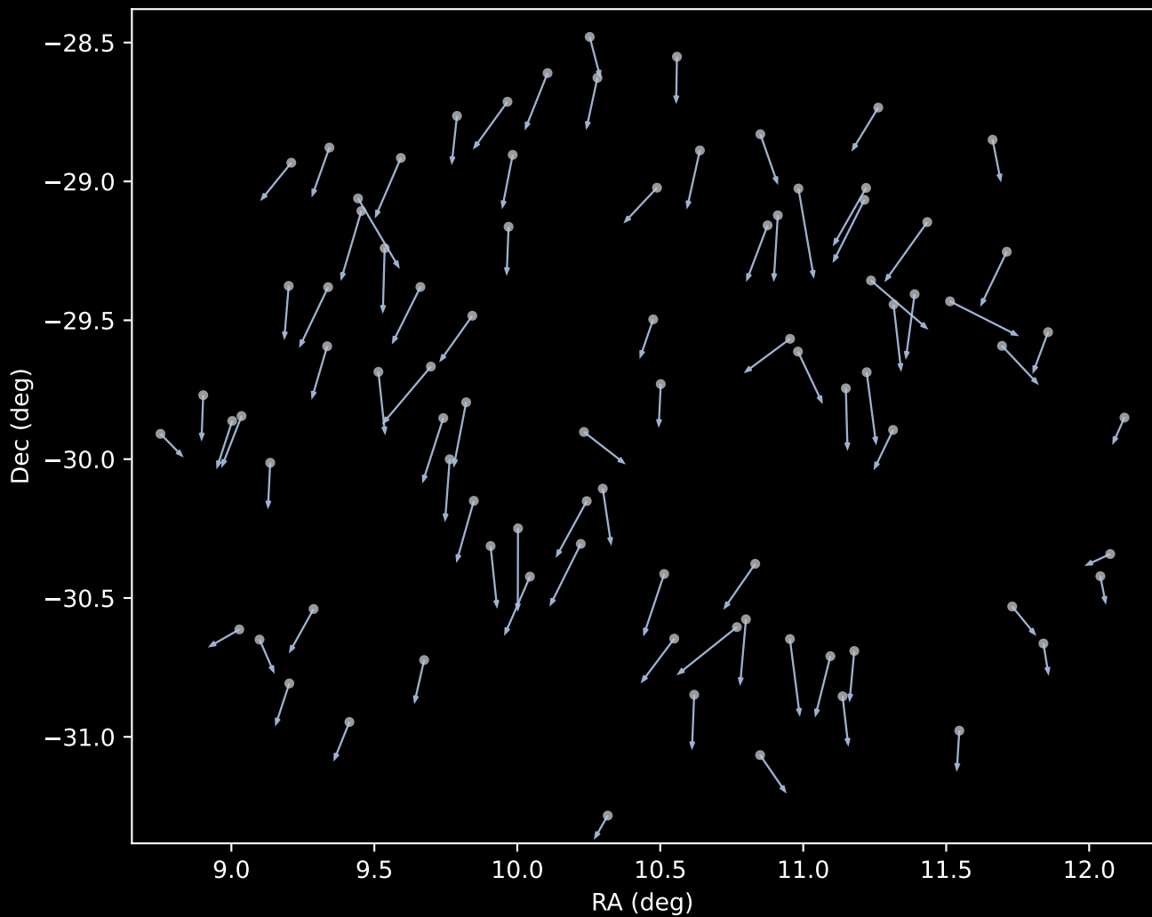
APOGEE DR17 Cluster 1 Proper Motion Vectors (n=86)
