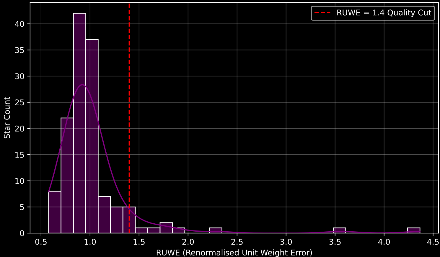
GAPOGEE DR17 Field [INTCL_N6528_MGA] RUWE Distribution (n= 134)
