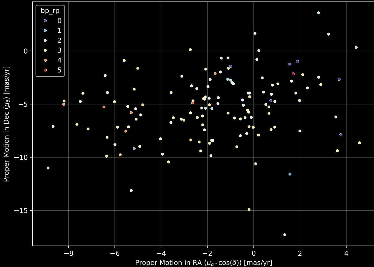
APOGEE DR17 Field: [INTCL_N6528_MGA] Proper Motion Diagram (n= 136)
