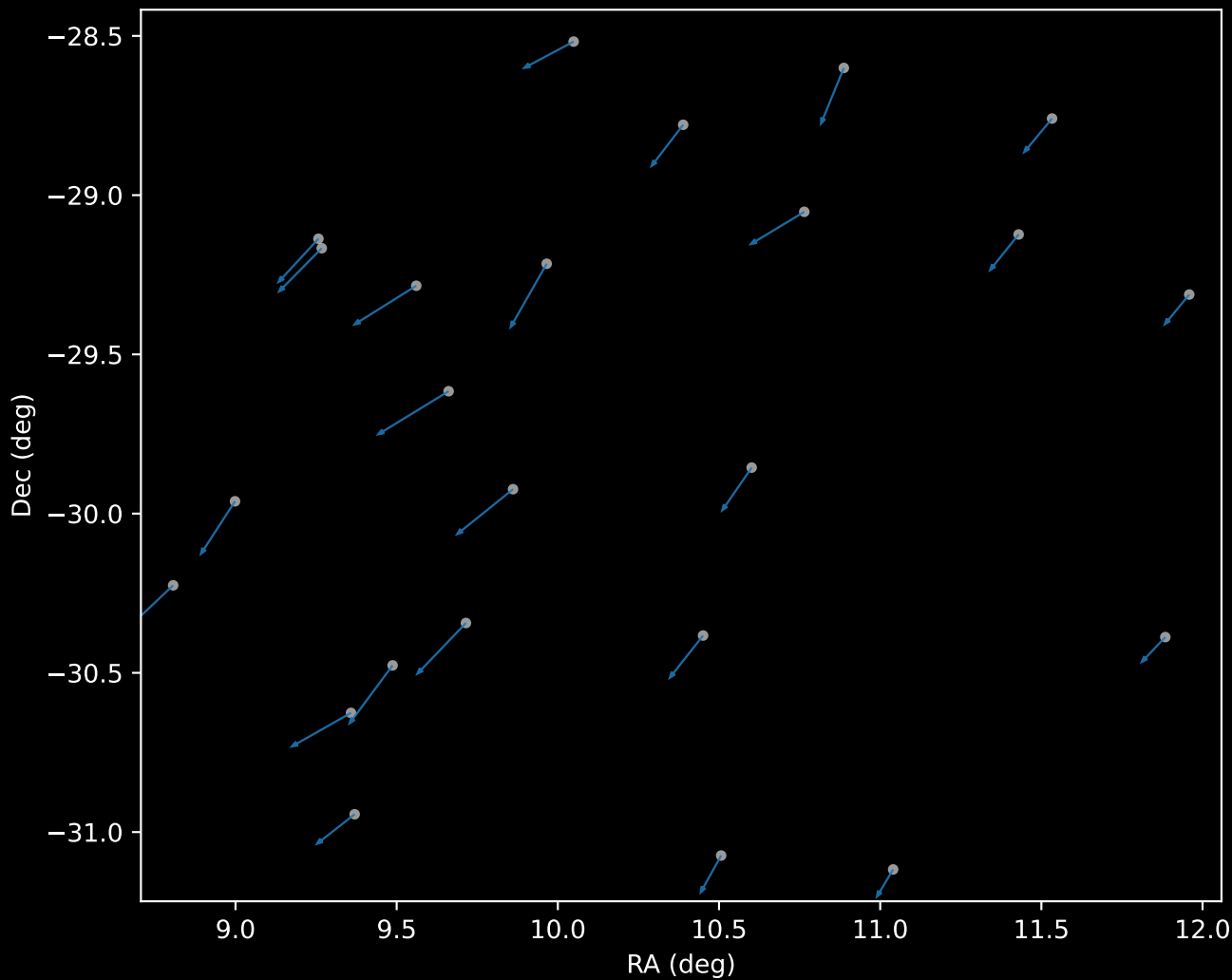
APOGEE DR17 Cluster 0 Proper Motion Vectors (n=24)
