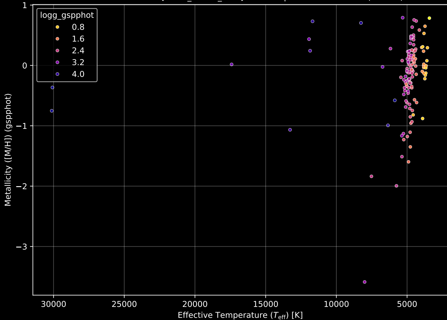
APOGEE DR17 Field: [INTCL_N6528_MGA] Stellar Population Parameters (n= 136)
