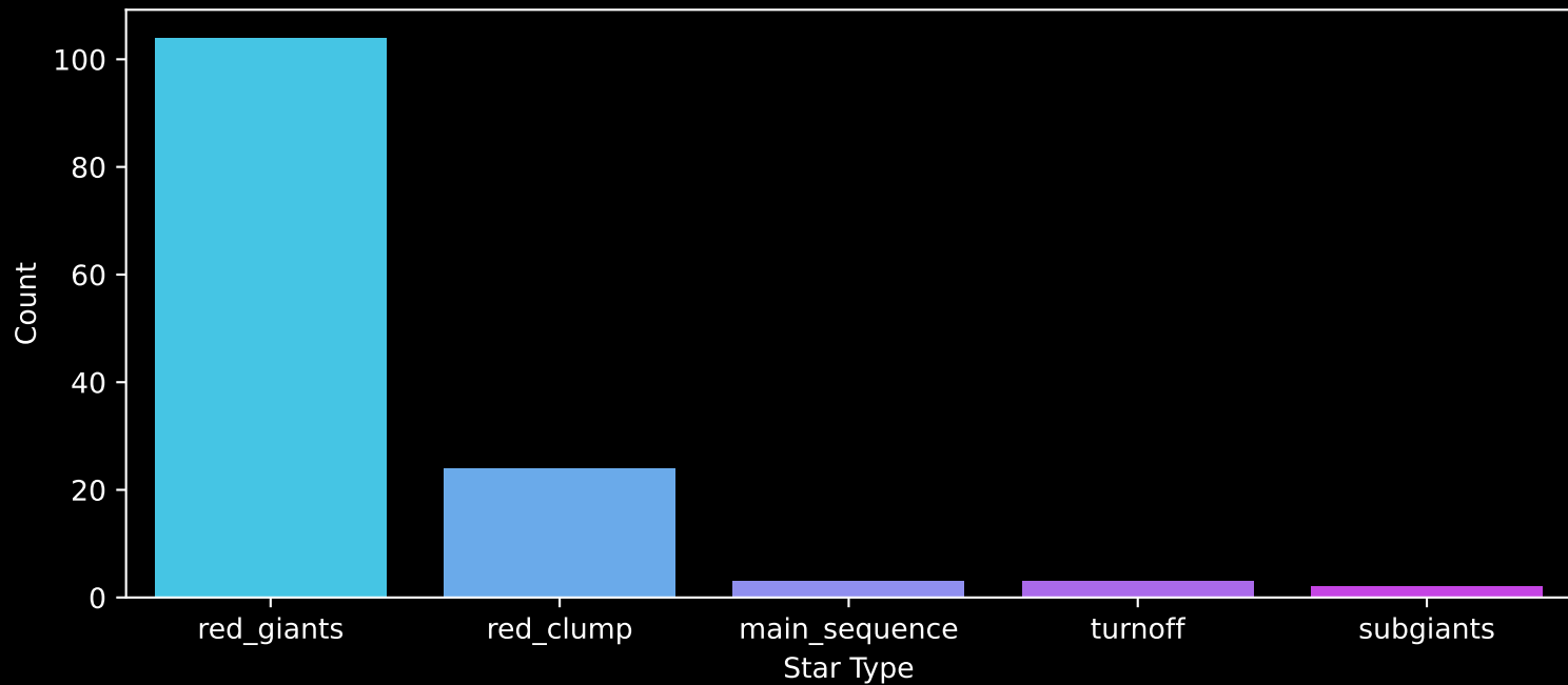
APOGEE DR17 Field: [INTCL_N6528_MGA] Count plot of Star Type
