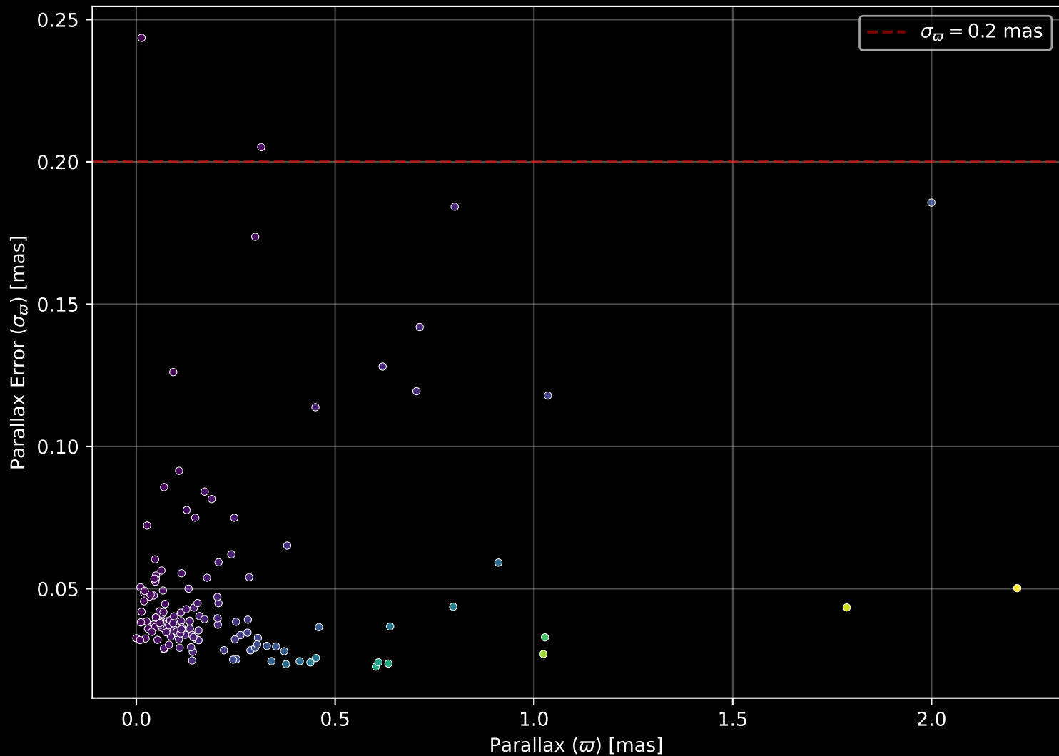
APOGEE DR17 Field: [INTCL_N6528_MGA] Parallax Quality (n= 136)
