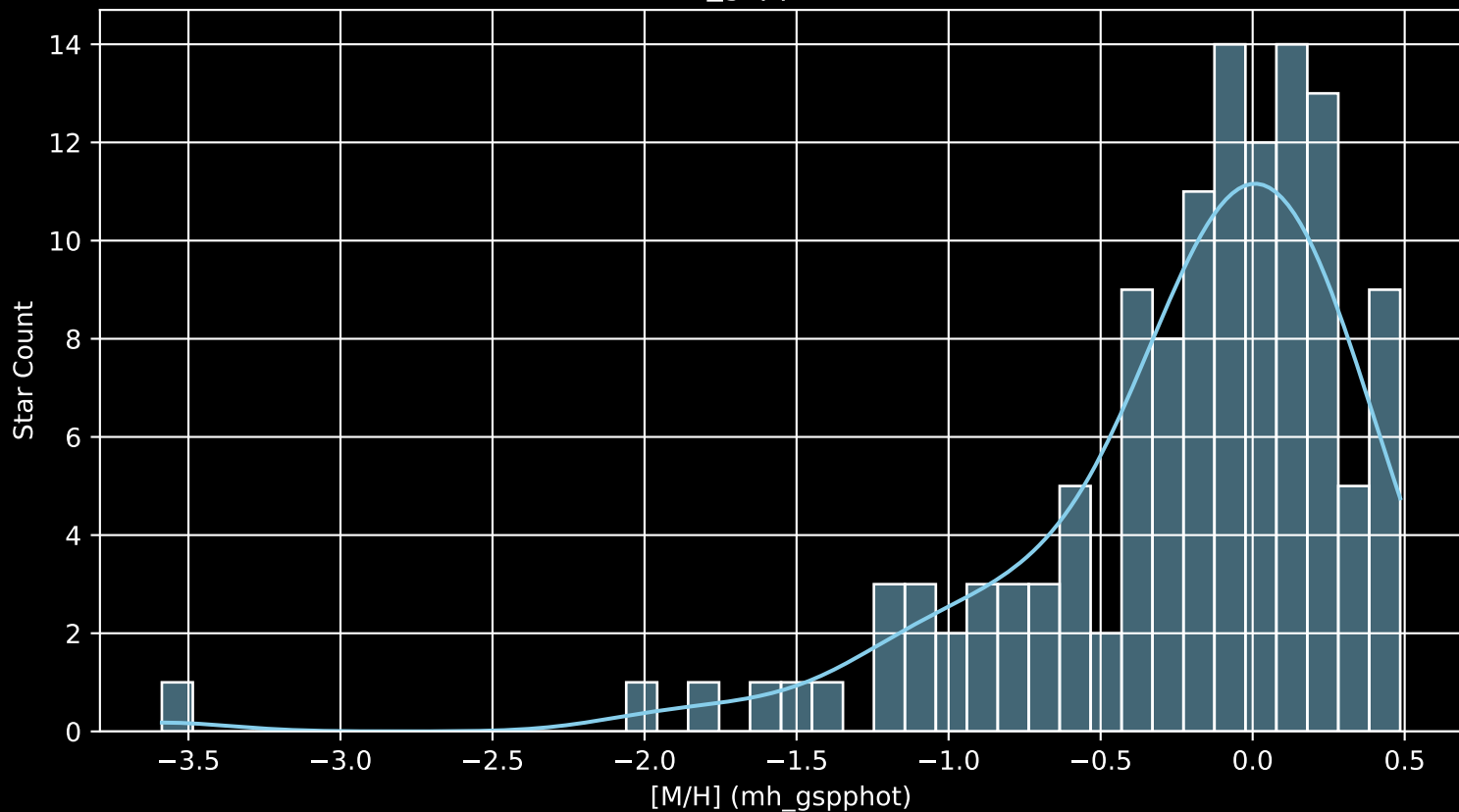
APOGEE DR17 Field: [INTCL_N6528_MGA [M/H] (mh_gspphot) (n= 125)
